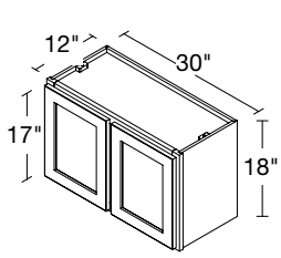
2 DOOR WALL BRIDGE 30" | W3018
