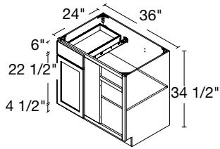
1 DOOR / 1 DRAWER BASE BLIND CORNER 36" | BBC36(L/R)
