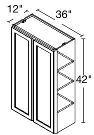
2 DOORS 36" | W3642
