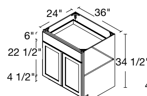
2 DOORS / 1 DRAWER 36" | B36
