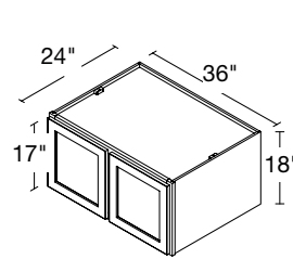
2 DOOR WALL BRIDGE 36" | W361824
