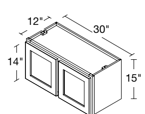
2 DOOR WALL BRIDGE 30" | W3015
