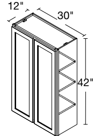
2 DOORS 30" | W3042
