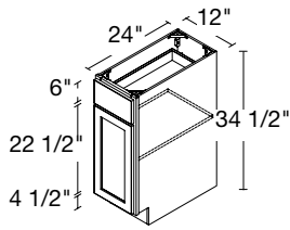
1 DOOR / 1 DRAWER 12" | B12(L/R)
