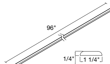
SCRIBE MOLDING 96 x 1/4 x 1 1/4" | SBM96
