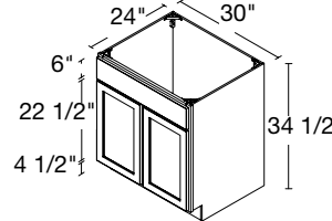
2 DOOR / 1 FALSE FRONT SINK 30" | SB30
