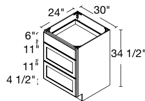
3 DRAWERS 30" | DB30
