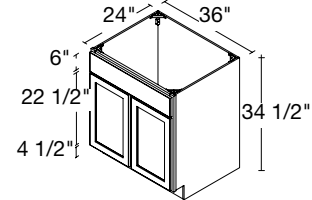
2 DOOR / 1 FALSE FRONT SINK 36" | SB36
