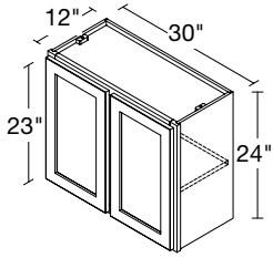
2 DOOR WALL BRIDGE 30" | W3024
