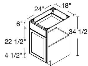
1 DOOR / 1 DRAWER 18" | B18(L/R)
