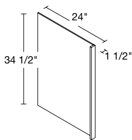
DISHWASHER END PANEL 1 1/2 x 34 1/2 x 24" DEP1.535
