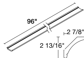
CROWN MOLDING 96 x 2 13/16 x 2 7/8" MCROWN8
