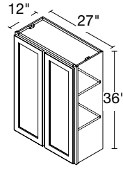
2 DOORS 27" | W2736
