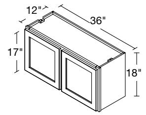
2 DOOR WALL BRIDGE 36" | W3618
