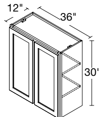
2 DOORS 36" | W3630
