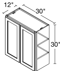
2 DOORS 30" | W3030
