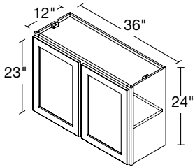
2 DOOR WALL BRIDGE 36" | W3624
