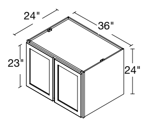
2 DOOR WALL BRIDGE 36" | W362424
