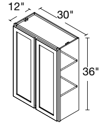
2 DOORS 30" | W3036
