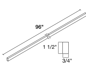
SQUARE EDGE MOLDING 96 x 3/4 x 1 1/2" | SEM96
