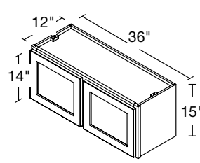
2 DOOR WALL BRIDGE 36" | W3615
