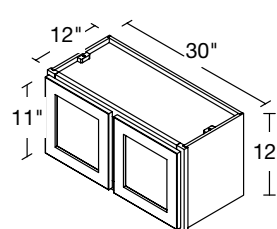
2 DOOR WALL BRIDGE 30" | W3012
