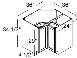
2 DOOR LAZY SUSAN BASE CORNER 36" | BC36LS
