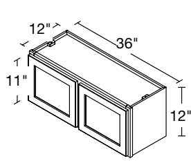
2 DOOR WALL BRIDGE 36" | W3612
