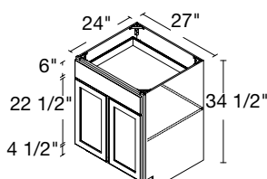
2 DOORS / 1 DRAWER 27" | B27
