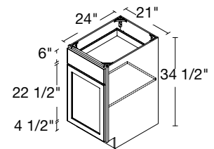
1 DOOR / 1 DRAWER 21" | B21(L/R)
