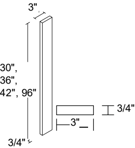
FILLER 3 x 3/4 x 30" | F330 3 x 3/4 x 36" | F336 3 x 3/4 x 42" | F342 3 x 3/4 x 96" | F396
