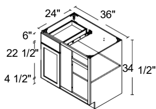
1 DOOR / 1 DRAWER BASE BLIND CORNER 36" | BBC36(L/R)
