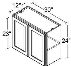
2 DOOR WALL BRIDGE 30" | W3024
