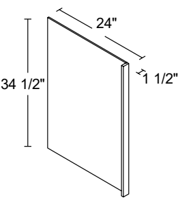
DISHWASHER END PANEL 1 1/2 x 34 1/2 x 24" DEP1.535
