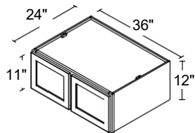
2 DOOR WALL BRIDGE 36" | W361224
