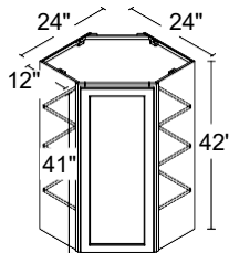
1 DOOR WALL CORNER 24" | WA2442(L/R)
