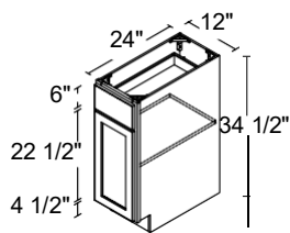
1 DOOR / 1 DRAWER 12" | B12(L/R)
