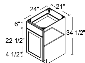
1 DOOR / 1 DRAWER 21" | B21(L/R)
