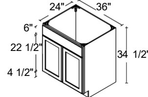
2 DOOR / 1 FALSE FRONT SINK 36" | SB36
