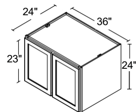
2 DOOR WALL BRIDGE 36" | W362424
