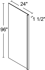
REFRIGERATOR END PANEL 1 1/2 x 96 x 24" REP2496
