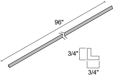
OUTSIDE CORNER MOLDING 96 x 3/4 x 3/4" | OCM96
