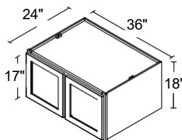
2 DOOR WALL BRIDGE 36" | W361824
