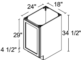
PULL-OUT WASTE CENTRE 18" | BWB18
