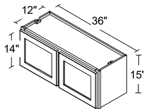
2 DOOR WALL BRIDGE 36" | W3615
