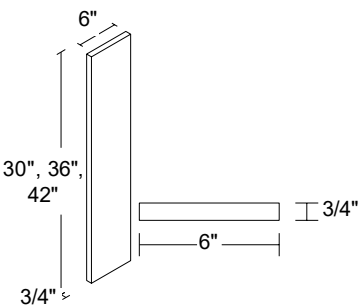
FILLER 6 x 3/4 x 30" | F630 6 x 3/4 x 36" | F636 6 x 3/4 x 42" | F642
