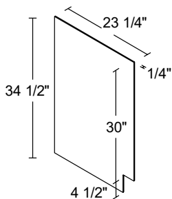
BASE END PANEL 1/4 x 34 1/2 x 23 1/4" BFEP2435
