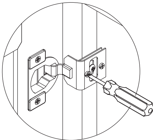
Left/Right Adjustment
