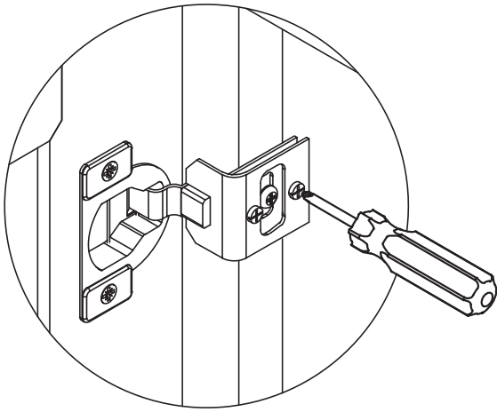
Front/Back Adjustment
