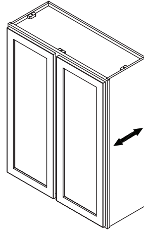
Front/Back Adjustment
