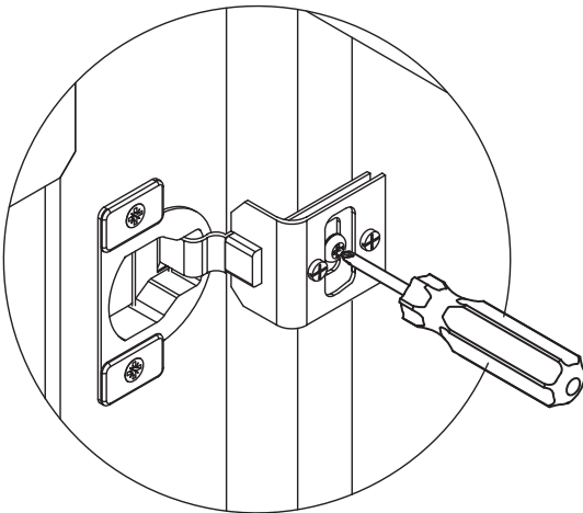
Up/Down Adjustment
